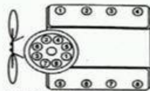
FORD MOTOR CO. V-8 221, 260, 289, 302 CID SMALL BLOCK 332, 352, 390, 406, 427, 428 CID FE SERIES 429, 460 CID BIG BLOCK
