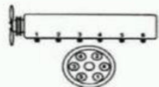
FORD MOTOR CO. 6 CYLINDER 144-300 CID (TYPICAL FOR EARLIER MODELS)
