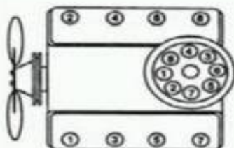
CHRYSLER CORP. V-8 273, 318, 340, 360 CID (SMALL BLOCK)
