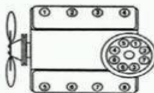
FORD MOTOR CO. V-8 239, 272, 292, 312 CID Y-BLOCK
