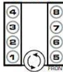
FORD 289, 302 FE, 429, 460
