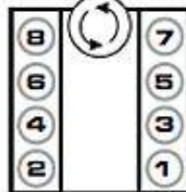
PONTIAC MOST V8
