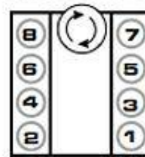
CHEVY (EXCEPT LS)
