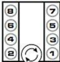
BUICK, MOST V8 EXCEPT NAIL HEAD
