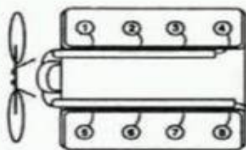
FORD MOTOR CO. 1932-48 FLATHEAD V-8 WIRES EMERGE FROM TUBES RUNNING ALONG INTAKE MANIFOLD
