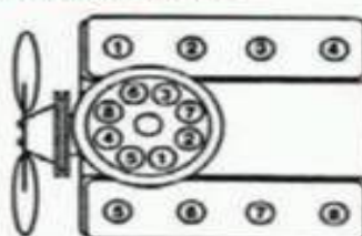
FORD MOTOR CO. 1949-53 FLATHEAD V-8
